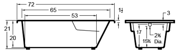
All bathtub dimensions are \pm 1/2" .
