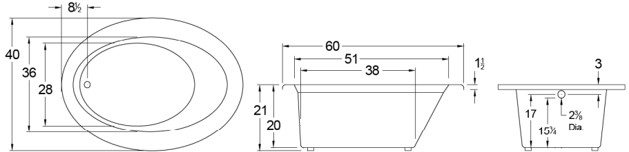
All bathtub dimensions are ± 1/2".
