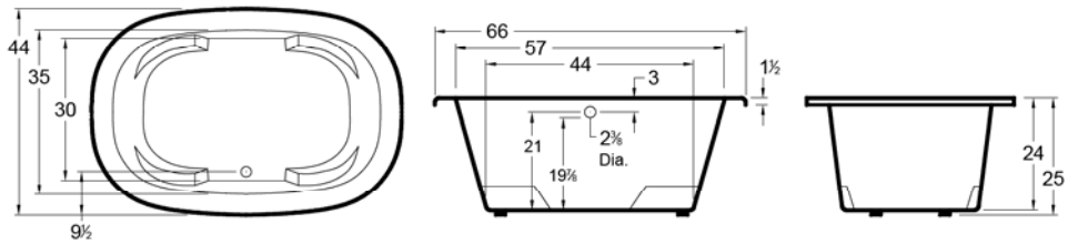
All bathtub dimensions are \pm 1/2'' .
